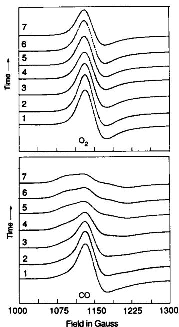
FIGURE 2 Effect of incubation at 233°K on the high-spin EPR spectrum (12°K, 0.01 M phosphate, pH 6.0) from 1,000 gauss to 1,300 gauss. (Top) The valency hybrid ( \alpha^+\beta^{02} )( \alpha^+\beta^{02} ) with both \alpha -chains oxidized and oxygen bound to the reduced chains, and (bottom) the hybrid ( \alpha^+\beta^0 )( \alpha^+\beta^0 ) with both \alpha -chains oxidized and carbon monoxide bound to the reduced chains. Before incubation, the EPR samples were stored in liquid nitrogen. Incubation at 233°K was performed in an external bath. After specified incubation times the EPR sample tube was placed in the EPR cavity. Incubation times: 1, 0 min; 2, 1 min; 3, 2 min; 4, 4 min; 5, 10 min; 6, 20 min; 7, 40 min.
