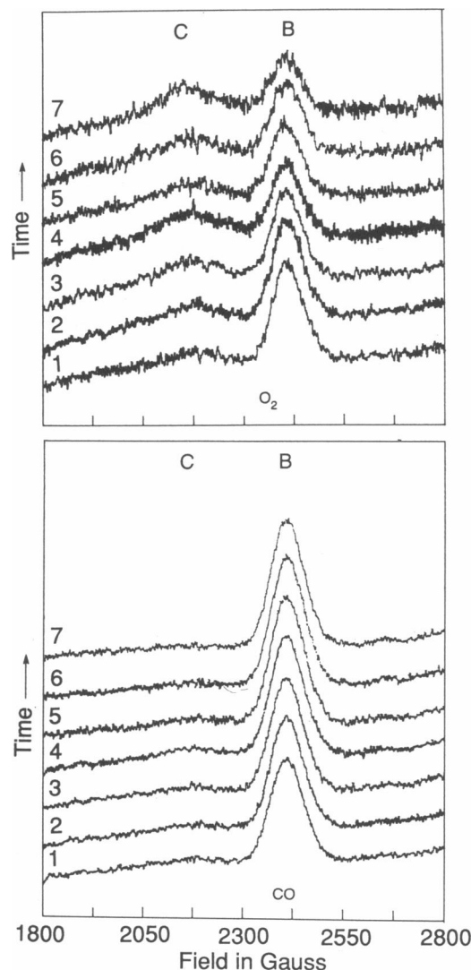
FIGURE 3 Effect of incubation at 233°K on the low-spin EPR spectrum (12°K, 0.01M phosphate, pH 6.0) from 1,800–2,800 gauss of the (Top) hybrid ( \alpha^+\beta^{02} )( \alpha^+\beta^{02} ) with both \alpha -chains oxidized and oxygen bound to the reduced chains, and (Bottom) the hybrid ( \alpha^+\beta^0 )( \alpha^+\beta^0 ) with both \alpha -chains oxidized and carbon monoxide bound to the reduced chains. Incubation times: 1, 0 min; 2, 1 min; 3, 2 min; 4, 4 min; 5, 10 min; 6, 20 min; 7, 40 min.
