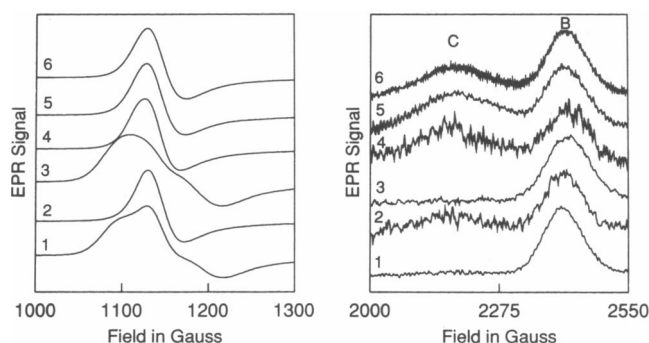
FIGURE 4 A comparison for different valency hybrids of the EPR spectra (12°K, 0.01 M phosphate, pH 6.0) obtained after incubation at 233°K. 1, (\alpha^+\beta^{\infty})(\alpha^+\beta^{\infty}) ; 2, (\alpha^+\beta^{02})(\alpha^+\beta^{02}) ; 3, (\alpha^{\infty}\beta^+)(\alpha^{\infty}\beta^+) ; 4, (\alpha^{02}\beta^+)(\alpha^{02}\beta^+) ; 5, (\alpha^+\beta^+)(\alpha^{\infty}\beta^{\infty}) ; 6, (\alpha^+\beta^+)(\alpha^{02}\beta^{02}) . (Left) The high-spin region of the EPR spectra from 1,000–1,300 gauss. (Right) The low-spin region of the EPR spectrum from 2,000–2,550 gauss.
